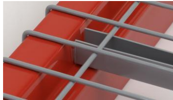
Standard U-Channel
